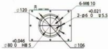
Installation flange
