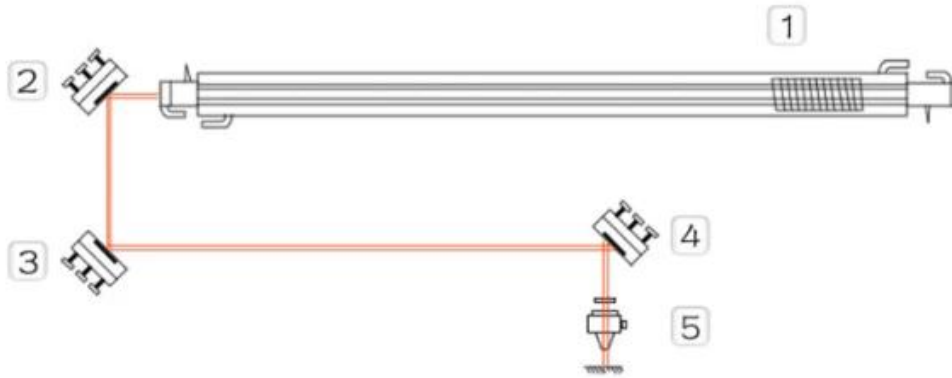
① Laser tube ② First mirror ③ Second mirror ④ Third mirror ⑤ Focus lens
