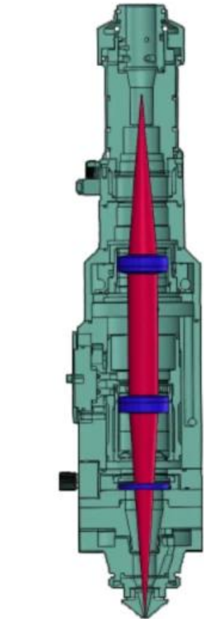
光纤切割头光路示意图 Figure of Fiber Cutting Head
